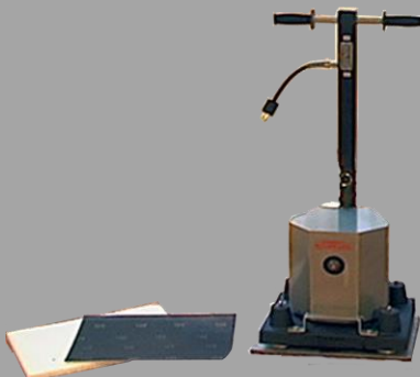
THE SL1218 ORBITAL REFINISHER 12" x 18" Orbital machine, 1Hp motor and larger flywheel work together to make the most aggressive unit in its class. The SL1218 is great for screen & re-coat jobs and exterior decks! Can also be used on other hard floor surfaces!
